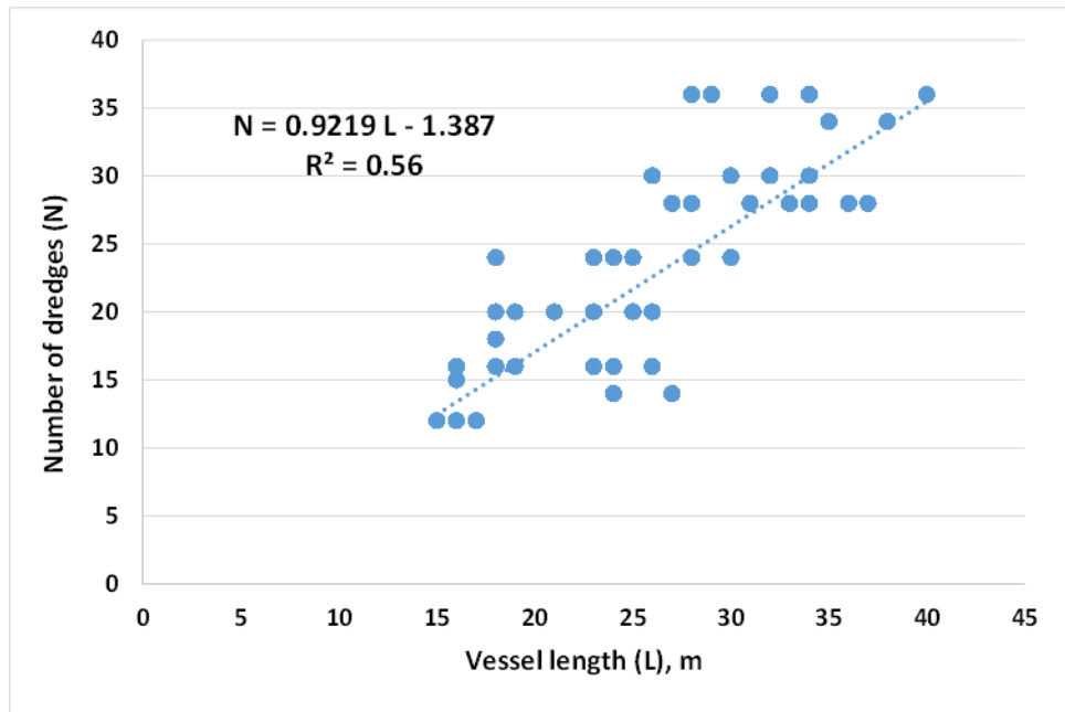
Figure 4 Correlation between number of dredges and vessel length for the UK fleet > 15 m.
