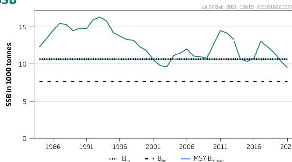
Figure 1 Sole in divisions 8.a–b. Summary of the stock assessment. Catches include discard estimates (no estimates between 2004 and 2015) and the assumed recruitment value for 2021 is shaded in a lighter colour.
