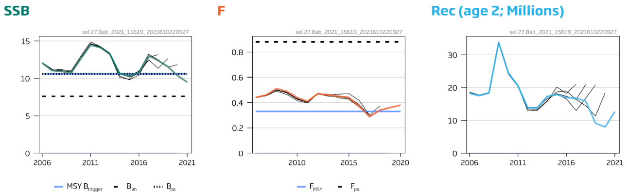
Figure 2 Sole in divisions 8.a–b. Historical assessment results (final-year recruitment assumptions included for each line).
