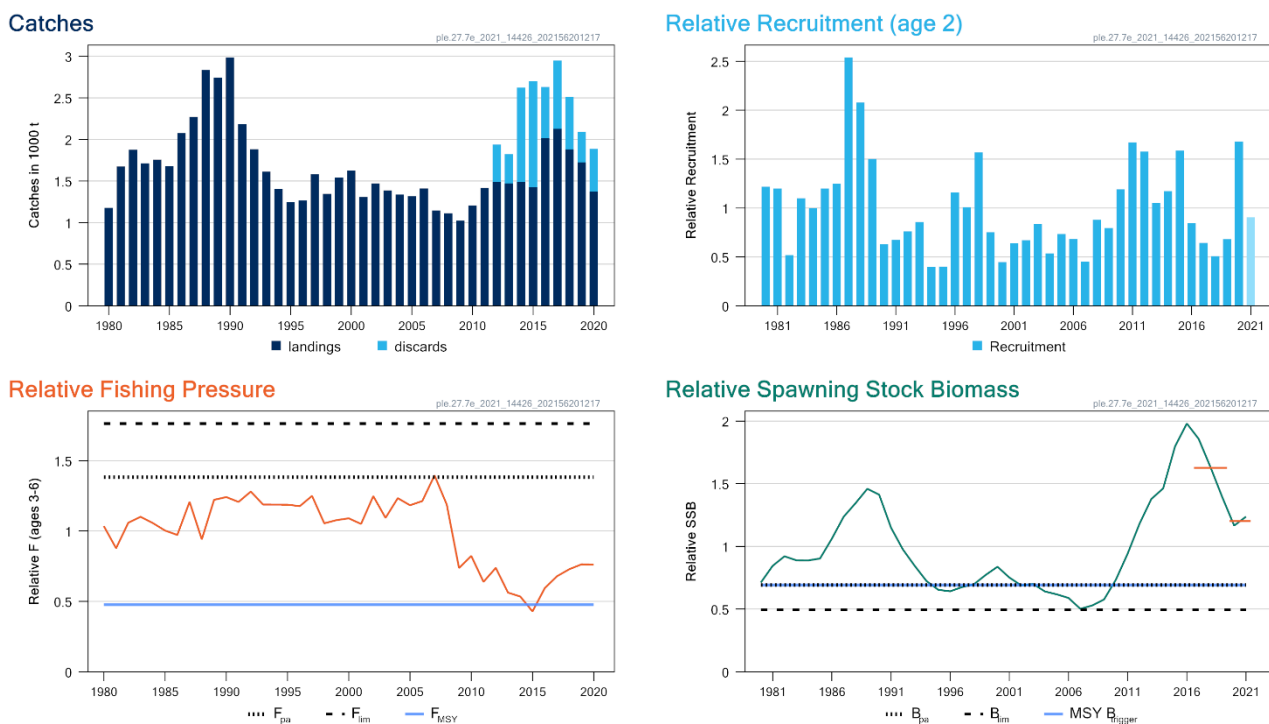
Figure 1 Plaice in Division 7.e. Summary of the stock assessment. Recruitment (R), fishing pressure (F), and spawning–stock biomass (SSB) are relative in relation to the average of the time-series. The assumed recruitment value for 2021 is shaded in a lighter colour. Discard data are only available from 2012 and are not included in the assessment. The orange horizontal lines indicate the average of the relative SSB index for 2017 to 2019 and for 2020 to 2021. All reference points are relative.
