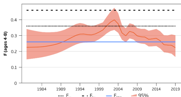
Figure 1 Mackerel in subareas 1–8 and 14, and in Division 9.a. Summary of the stock assessment. The paler shaded catches prior to 2000 have been down-weighted in the assessment because of the considerable underreporting suspected to have taken place in this period. The recruitment value for 2019 is estimated using the recruitment survey (IBTS) and a model (RCT3), and the recruitment value for 2020 is the geometric mean of the recruitments from 1990 to 2018.
