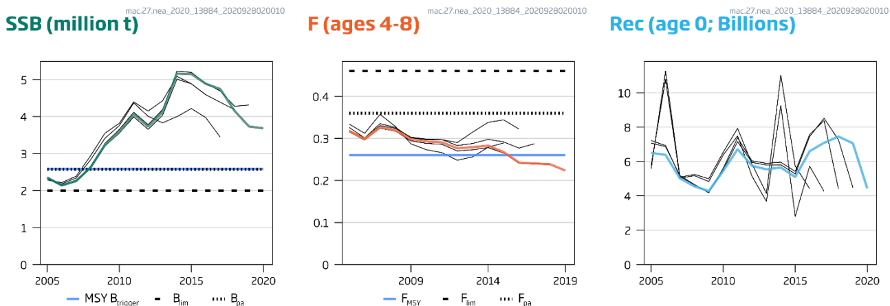
Figure 2 Mackerel in subareas 1–8 and 14, and in Division 9.a. Historical assessment results. Since the 2014 assessment, the last year of each recruitment line is the assumed value used in the forecast. Reference points have been revised in 2020.
