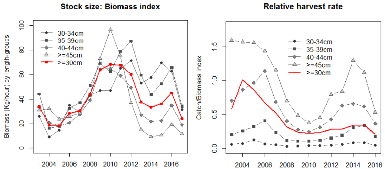
Figure 3 Cod in subdivisions 24–32, eastern Baltic stock. Left panel: Stock size indicator by length groups and overall index \geq 30 cm (note: the index of biomass \geq 30 cm is the same as the one shown in Figure 1, but rescaled in order to facilitate visual comparison). Right panel: Mean relative harvest rate (total catch divided by stock size indicator for \geq 30 cm cod; red line) compared with relative harvest rates for individual length groups.
