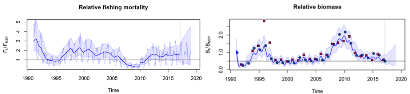
Figure 2 Cod in subdivisions 24–32, eastern Baltic stock. SPiCT model results used for the evaluation of the stock and exploitation status (the proxy F_{MSY} and MSY\ B_{trigger} are represented by horizontal lines in the left and right panels, respectively).
