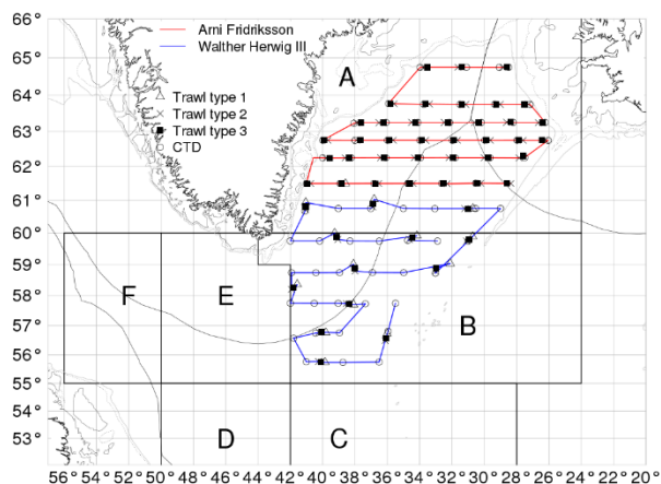
Figure 2.3.4b.2 Beaked redfish in Subareas V, XII, and XIV and NAFO Subareas 1+2 (shallow pelagic stock < 500 m). Survey cruise tracks in the international redfish survey in June/July 2015. Areas C–E are normally covered in this survey, but were not surveyed in 2015 and no biomass estimate could be obtained for the stock.
