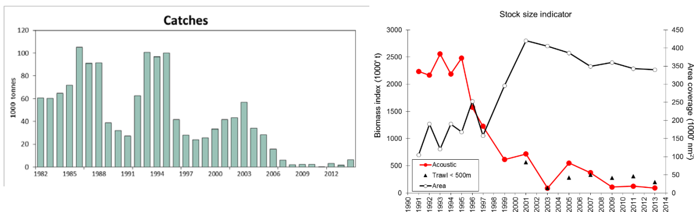
Figure 2.3.4b.1 Beaked redfish in Subareas V, XII, and XIV, and NAFO Subareas 1+2 (shallow pelagic stock < 500 m). Left: Catches (tonnes). Right: Results of acoustic survey indices (thousand tonnes) from above the scattering layer (red filled circle), trawl estimates within the scattering layer and shallower than 500 m (black triangle), and aerial coverage (NM 2 ) of the survey (black open circle) in the Irminger Sea and adjacent waters. No survey biomass estimates were available in 2015 due to insufficient coverage.
