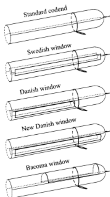
Figure 12. Variations of codend with square mesh windows tested in the Baltic Cod fishery.
