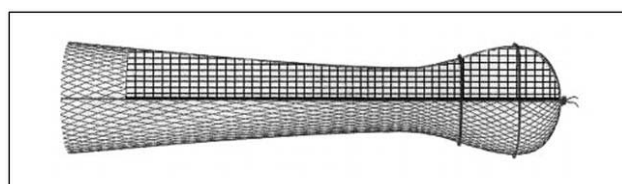
Figure 11. Composite codend showing square-mesh netting covering the top portion of the codend and diamond-mesh netting on the bottom half.
