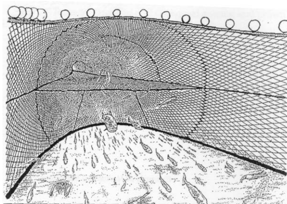
Figure 6. Horizontal Separator Panel
