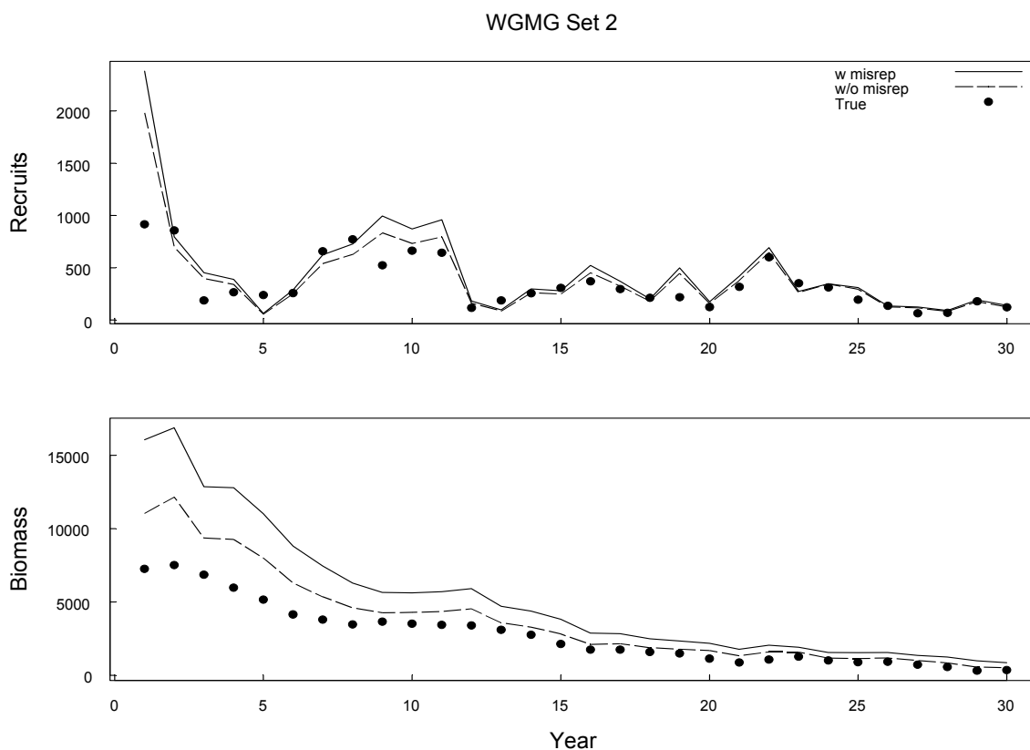
Figure 4.3.2.4.4. CSA analysis of set 2. Estimates of recruitment (top) and biomass (bottom) compared to the truth (solid circles), and to an analysis of the same data without misreporting (dashed line).
