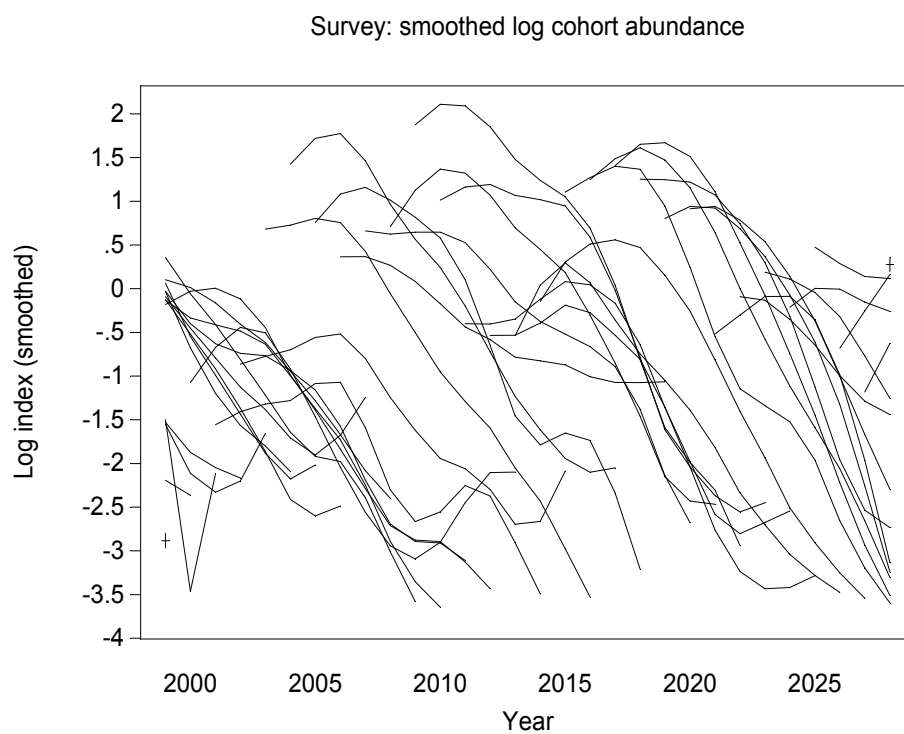
Figure 4.2.1.3. Smoothed catch curves from dataset 1 (see Section 4.3.1).
