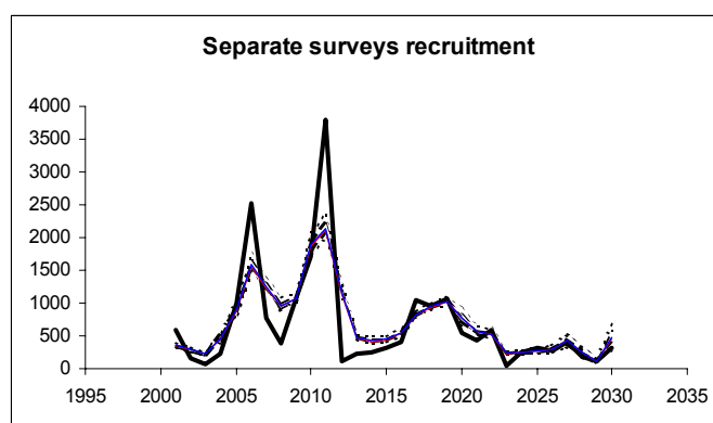
Figure 4.3.2.9.6c .The time-series of XSA estimated bootstrap percentiles of recruitment mortality estimated for the fit to the split Data Set 1 survey time-series. The bold line presents the truth.
