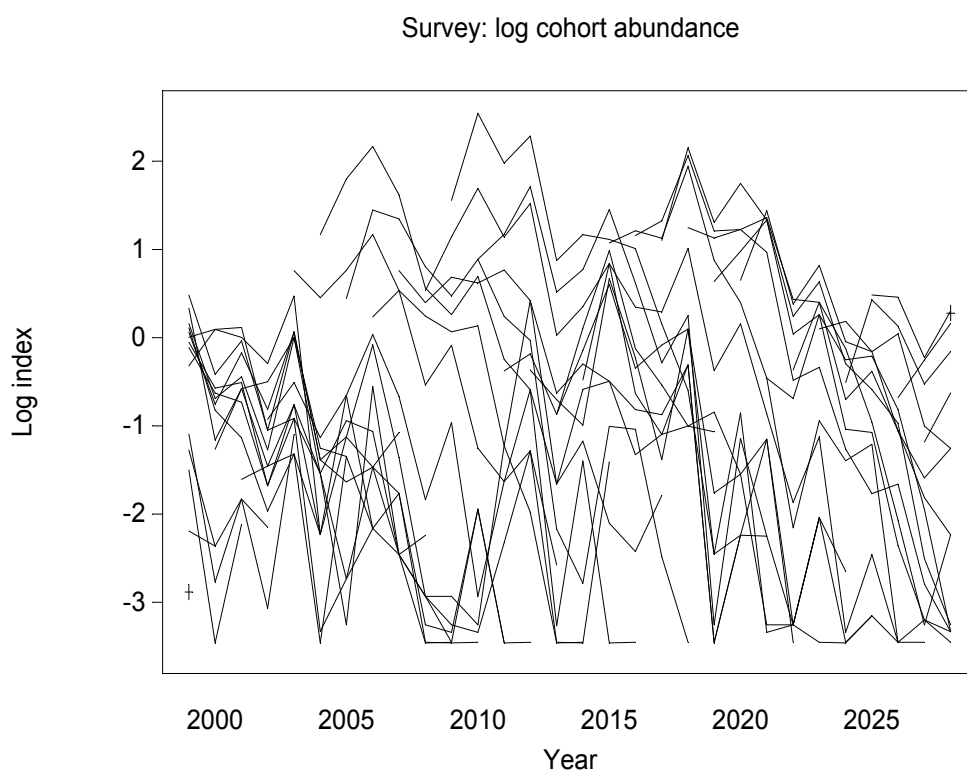
Figure 4.2.1.2. Raw catch curves from dataset 1 (see Section 4.3.1).
