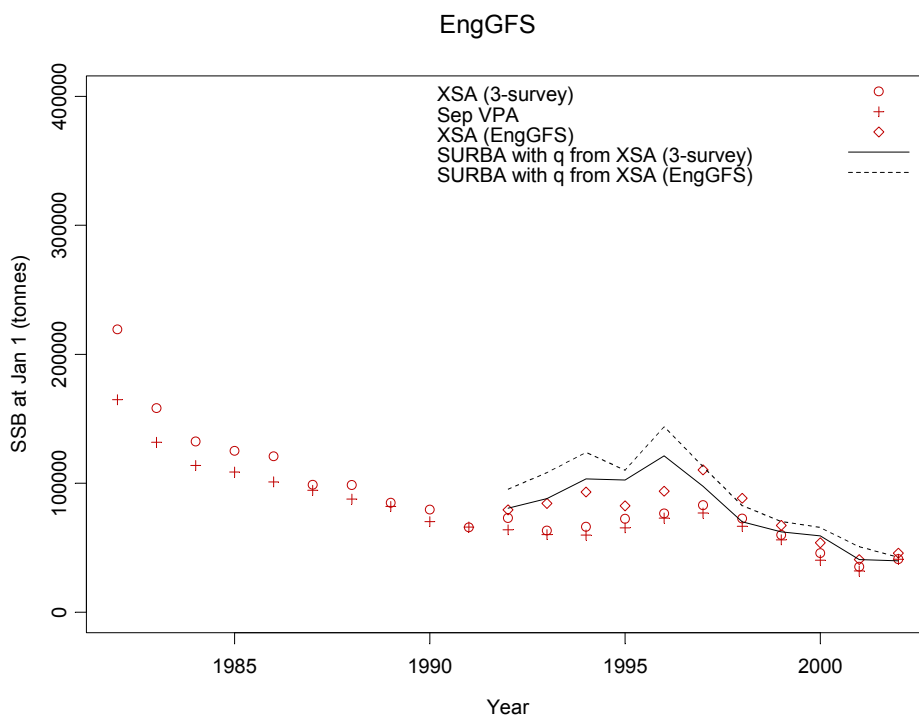
Figure 10. North Sea cod. Comparison of absolute SSB estimates from XSA, SURBA and separable VPA runs. See text for details.
