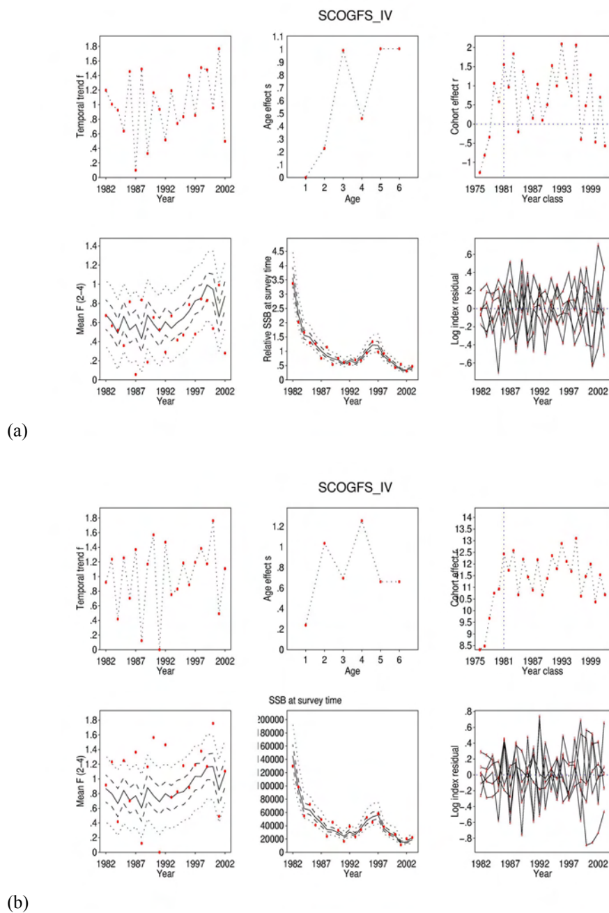
Figure 6. SURBA analysis summary examples for the Scottish groundfish survey on North Sea cod, using (a) relative abundance estimation, and (b) absolute abundance estimation. See caption to Figure 1 for key.
