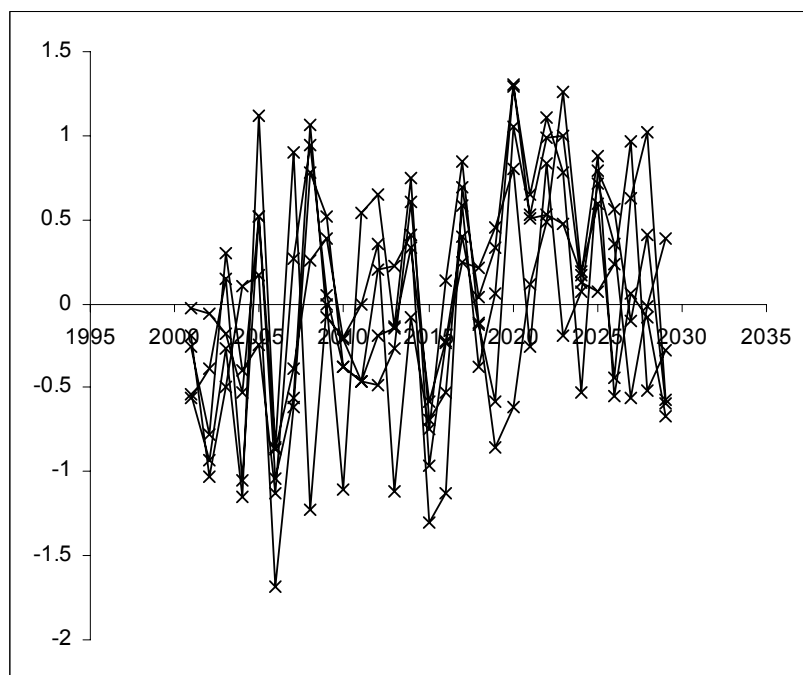
Figure 4.3.2.9.3. The time-series of Data Set 1 survey CPUE log catchability residuals at ages 4 – 9 from a Laurec Shepherd tuning. The patterns indicate departure from the assumption of constant catchability after 2015.
