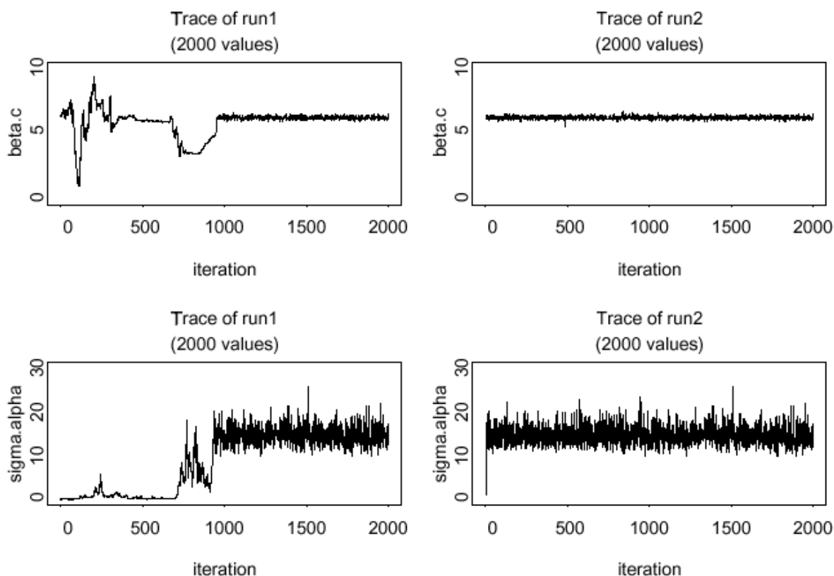
Figure 4.2.2.2.1. Bayesian sample chains.
