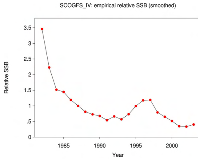
Figure 5. Empirical plots of (a) \bar{Z}_{2-4} and (b) relative SSB at survey time for the Scottish groundfish survey on North Sea cod.
