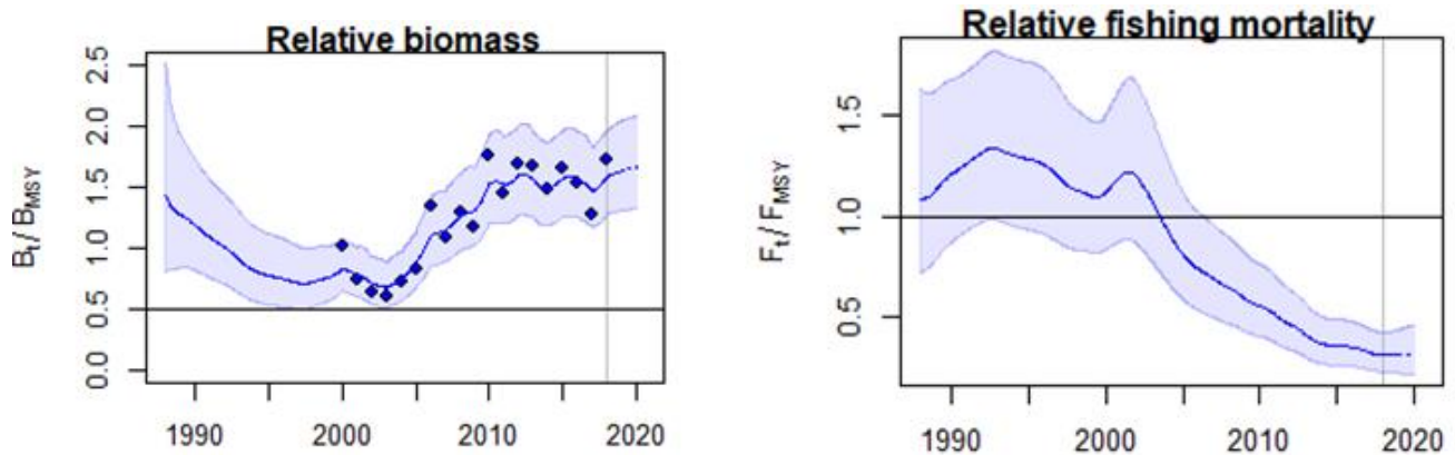
Figure 2 Tusk in subareas 4 and 7–9, and in divisions 3.a, 5.b, 6.a, and 12.b. SPiCT model results used for the evaluation of the stock and exploitation status. The horizontal lines indicate the reference points B_{trigger\_proxy} and F_{MSY\_proxy} .
