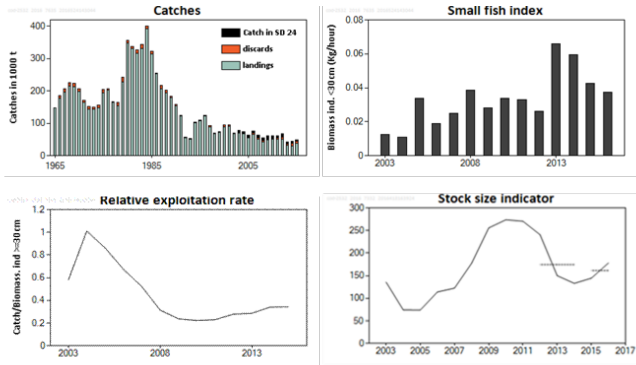
Figure 8.3.5.1 Cod in subdivisions 24–32 (eastern Baltic cod). Upper left panel: catches in subdivisions 25–32+24 (in thousand tonnes), divided in ICES estimated landings and discards, and catches of the eastern Baltic cod stock taken in Subdivision 24. The EU landing obligation started in 2015; therefore, landings in 2015 include fish above and below the minimum conservation reference size (MCRS). Upper right panel: small fish index, calculated as cpue (kg hour -1 ) of fish < 30 cm from the 1st and 4th quarters, from the BITS survey in subdivisions 25–28. Lower left panel: relative exploitation rate (catches of the eastern Baltic cod stock/stock size indicator). Lower right panel: stock size indicator, calculated as cpue (kg hour -1 ) of fish ≥ 30 cm from the 1st and 4th quarters, from the BITS survey in subdivisions 25–28. The dashed lines in the relative SSB plot indicate the average values of the respective years.
