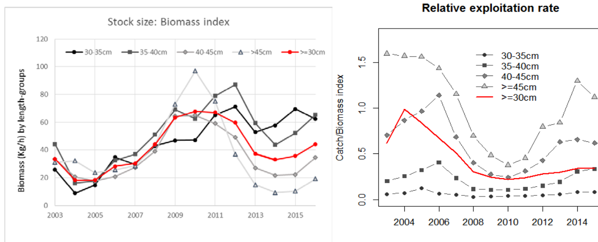
Figure 8.3.5.2 Cod in subdivisions 24–32 (eastern Baltic cod). Left panel: Stock size indicator by length groups and overall index \geq 30 cm (note: the index of biomass \geq 30 cm is the same one as shown in Figure 8.3.5.1, but rescaled in order to facilitate visual comparison). Right panel: Mean relative exploitation rate (total catch divided by stock size indicator for \geq 30 cm cod; red line) compared with relative exploitation rates for individual length groups.
