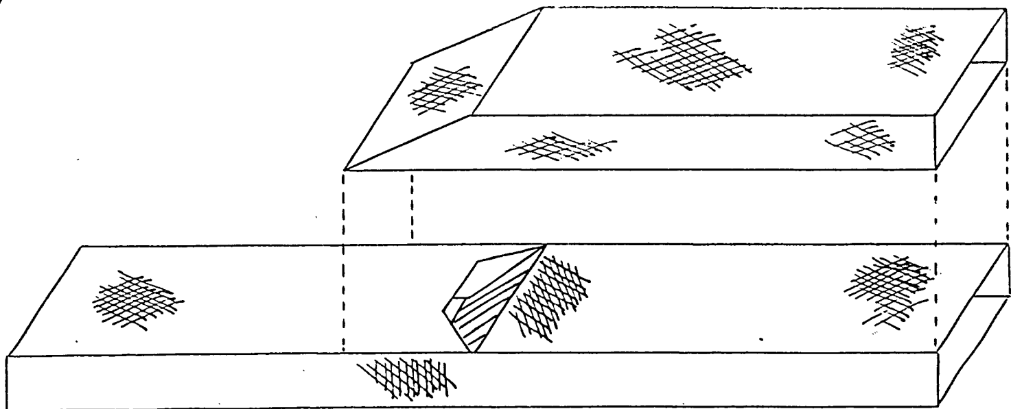
Figure 2: Diagrams showing the two-codend selective trawl with the grid ( vertical bars) and the trap for the larger fish.
