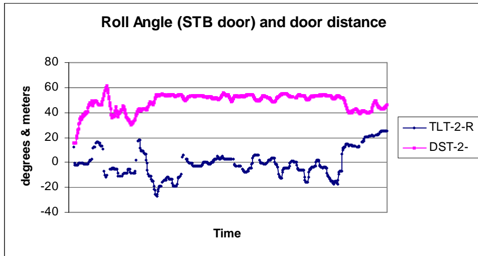
Figure 3.2.5: Measurements of roll (starboard door, lower curve; below zero- door heeling inward, above zero-door heeling outward) and door spread (upper curve (m)).
