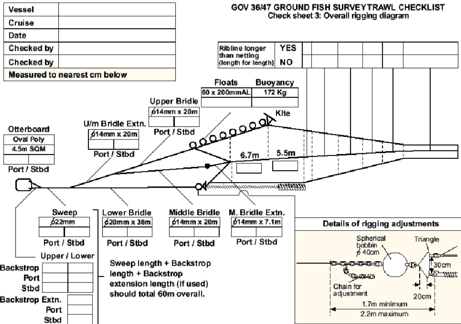
Figure 4.4.2: Rigging check list for the 36/47 GOV Trawl.
