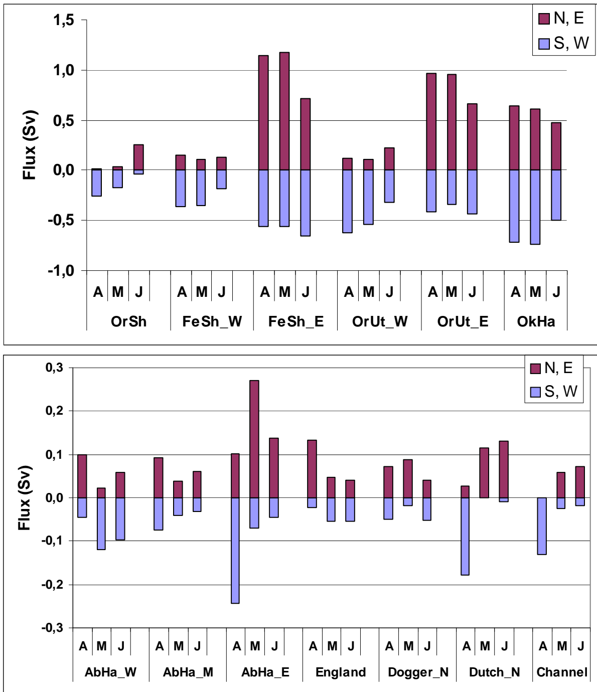
Figure 4. The mean monthly water fluxes for April, May, and June 2007 across sections in the North Sea (see Figure 2 for their locations). NORWECOM model estimates. Positive values denote northwards or eastwards transport while negative values denote southwards or westwards transport.
