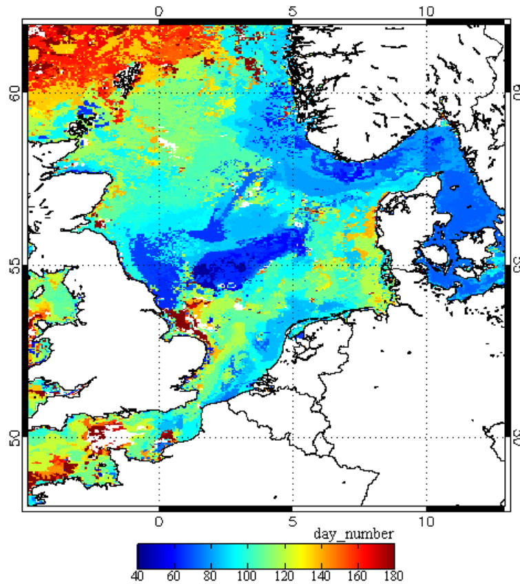
Figure 18. Algae bloom timing (based on seasonal chlorophyll build-up) for the North Sea in the year 2007 derived from MERIS and MODIS data. White areas denote land and pixels where no bloom was detected in first half of year. Chlorophyll data was received from ACRI-ST in the framework of the GMES-MARCOAST project (and ESA Cat 1 A/O 1521) and processed by MUMM using the method of Park and Ruddick (2007).
