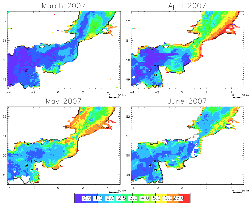
Figure 17. Monthly mean chlorophyll a concentration in March–June 2007 derived from ENVISAT-MERIS for the Southern Bight of the North Sea and the Channel. White areas denote land and pixels where no acceptable satellite data was available (because of clouds or failure of quality control checks). Belgian waters are delineated by the thin grey lines. Data provided by the European Space Agency in the framework of Envisat AOID 698, processed by MUMM (BELCOLOUR project).
