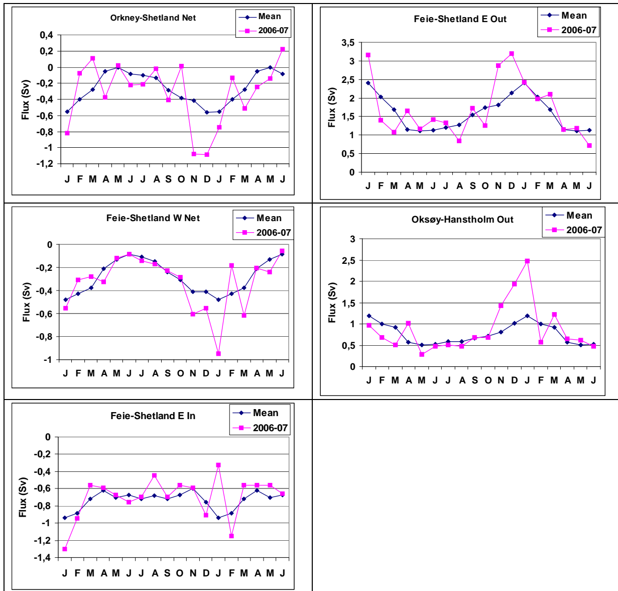
Figure 5. Modelled fluxes of water across sections in the northern North Sea and in the Skagerrak (see Figure 2 for their locations). The mean monthly fluxes from January 2006 to June 2007 are shown along with the long-term mean (1955–2004) monthly fluxes. Net flux is the difference between northwards and southwards fluxes for transects oriented in the E-W direction, and between eastwards and westwards fluxes for transects oriented in the N-S direction. In and Out are used to denote southwards and northwards fluxes into and out of the North Sea across the northern boundaries. Out for the Oksøy-Hanstholm section denotes outflow from Skagerrak. Negative values are southwards and westwards fluxes, while positive values are northwards and eastwards fluxes for E-W and N-S oriented sections, respectively.
