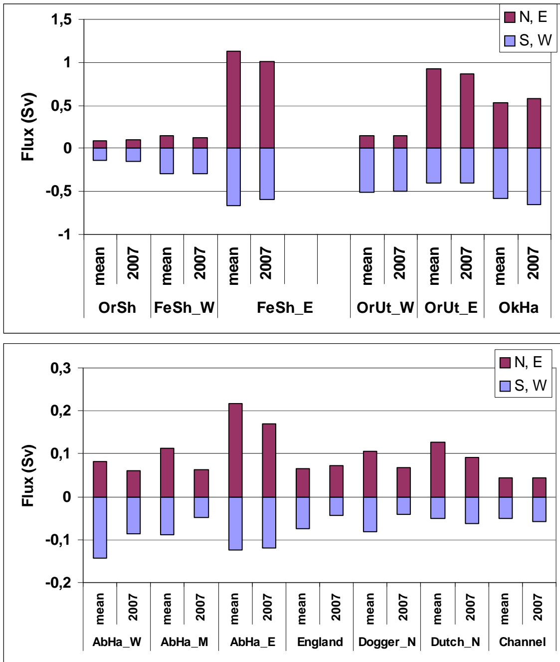
Figure 3. The 2007 mean 2 nd quarterly water fluxes across sections in the North Sea compared to the long-term mean fluxes for the 2 nd quarter (1955–2004). NORWECOM model estimates. See Figure 2 for the location of the sections. Positive values denote northwards or eastwards transport while negative values denote southwards or westwards transport.
