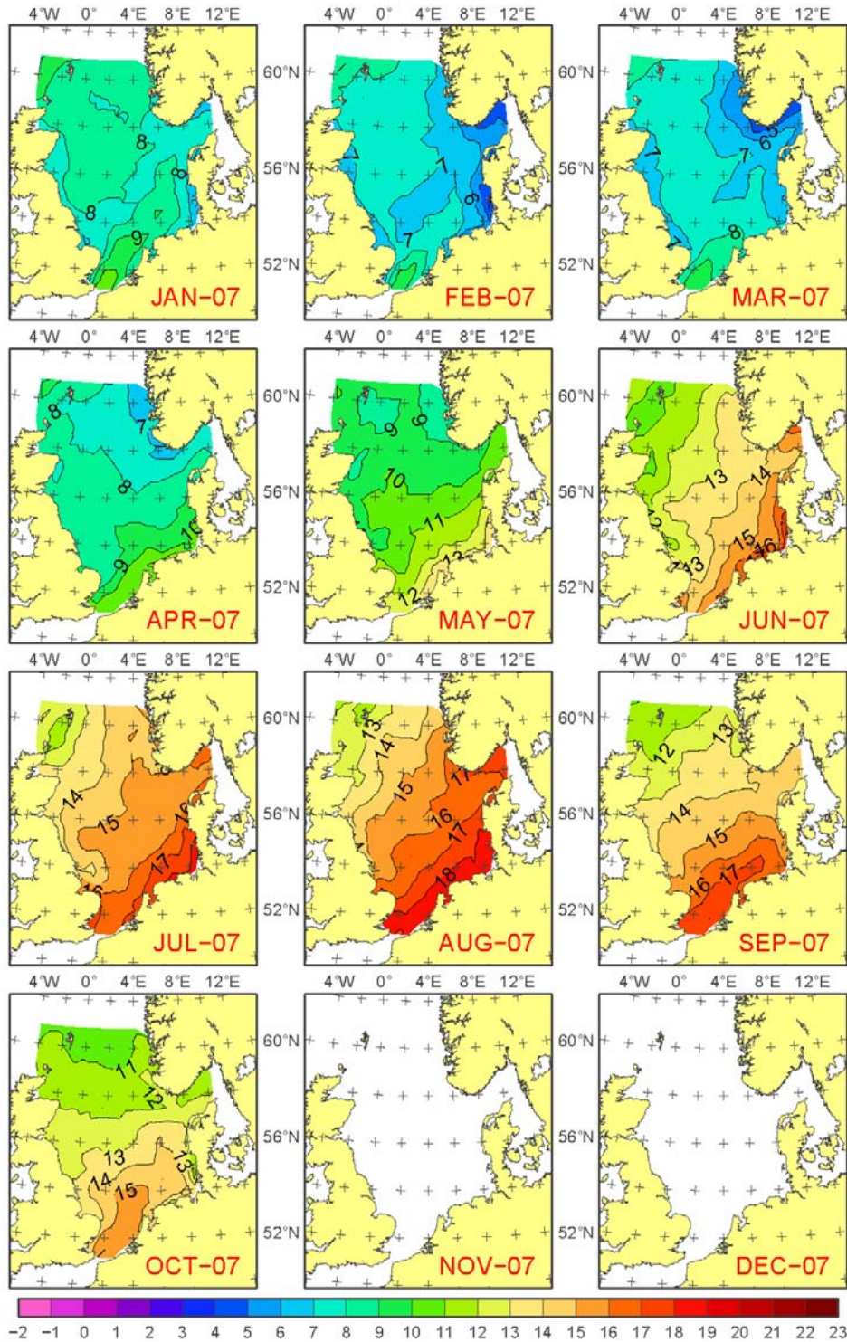
Figure 8. Monthly mean sea surface temperature for January–October 2007. Data from BSH, Hamburg.
