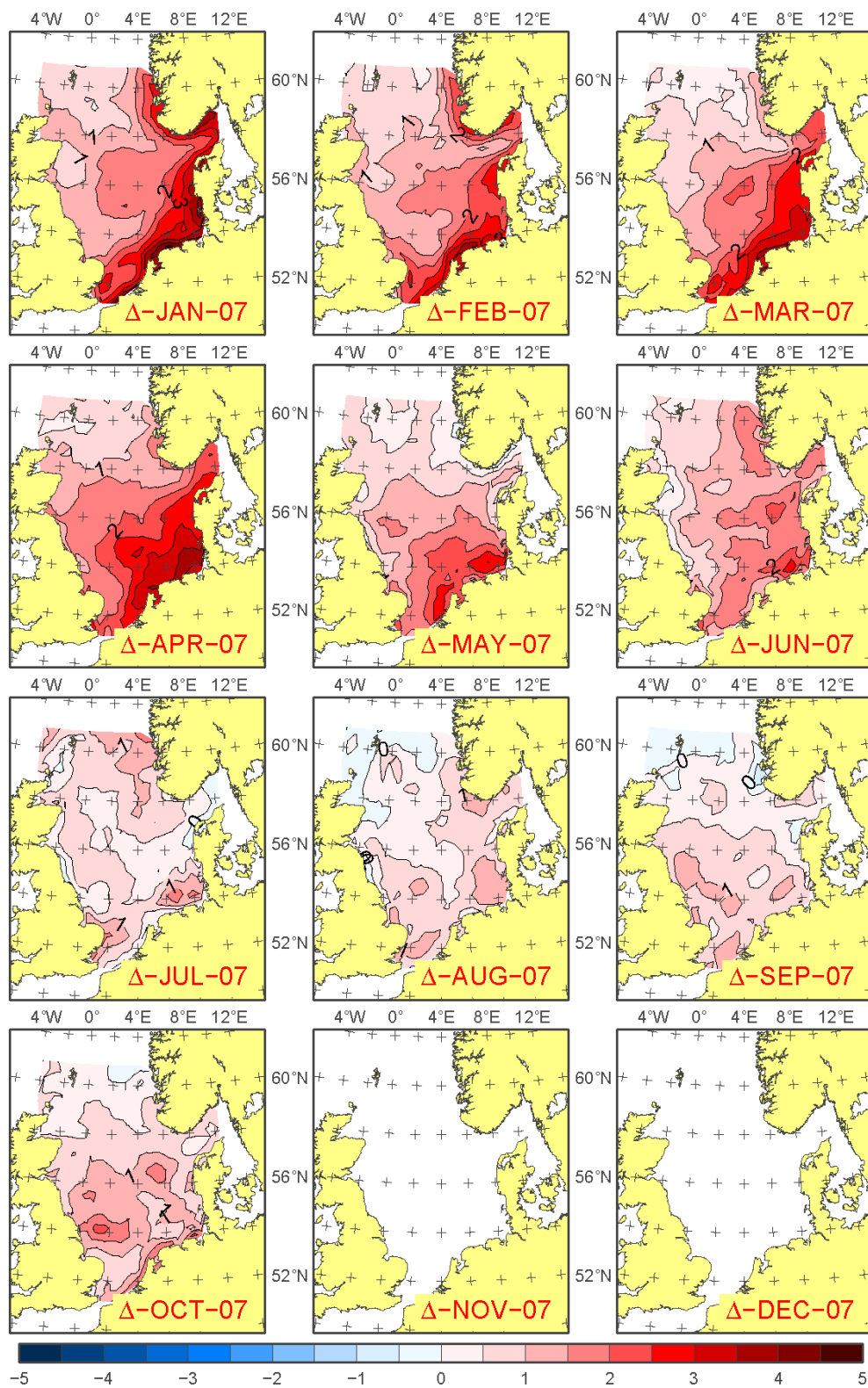
Figure 9. Anomalies for monthly mean sea surface temperature for January – October 2007. Data from BSH, Hamburg.
