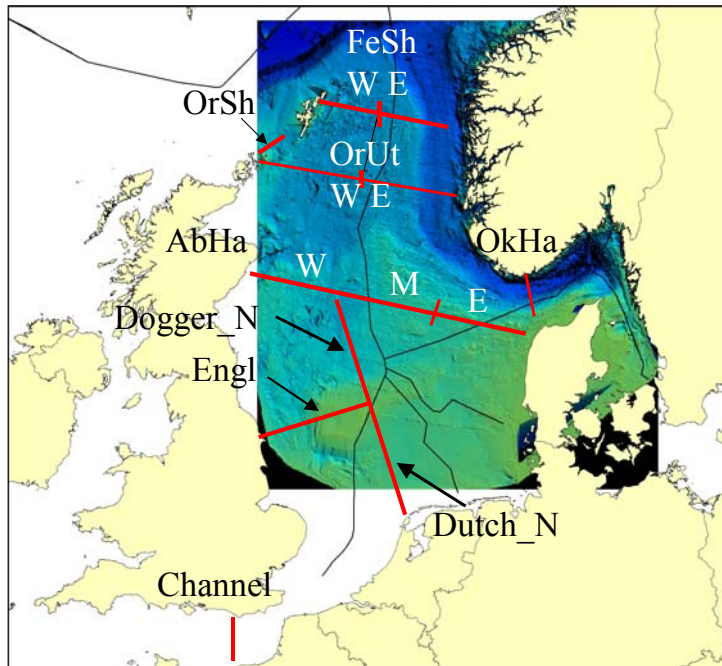
Figure 2. Sections across various parts of the North Sea used to calculate fluxes of water with the 3-D mathematical circulation model NORWECOM.
