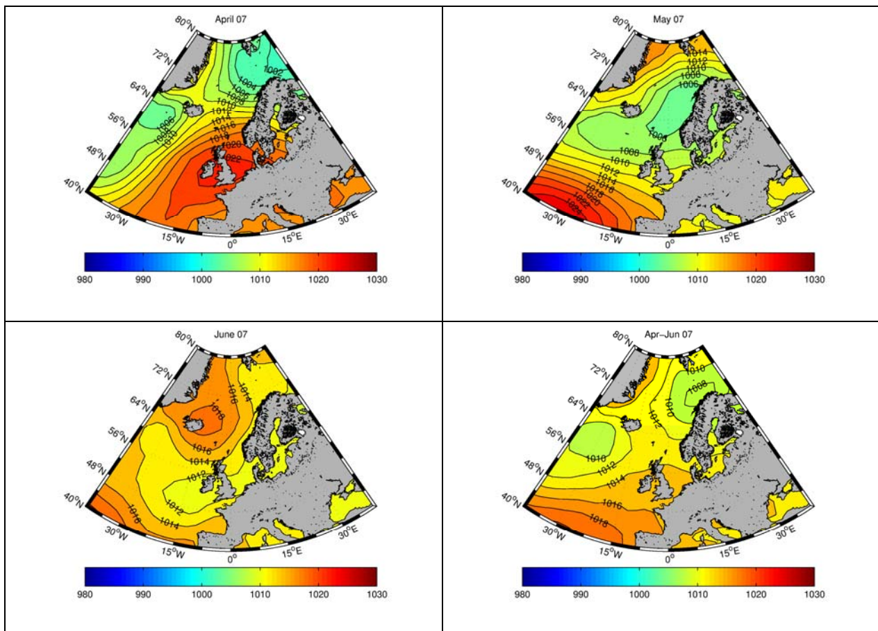
Figure 1. Monthly mean sea level air pressures for April, May, and June 2007 (upper left and right, and lower left panels) and the mean for the 2 nd quarter (April–June) 2007 (lower right panel).
