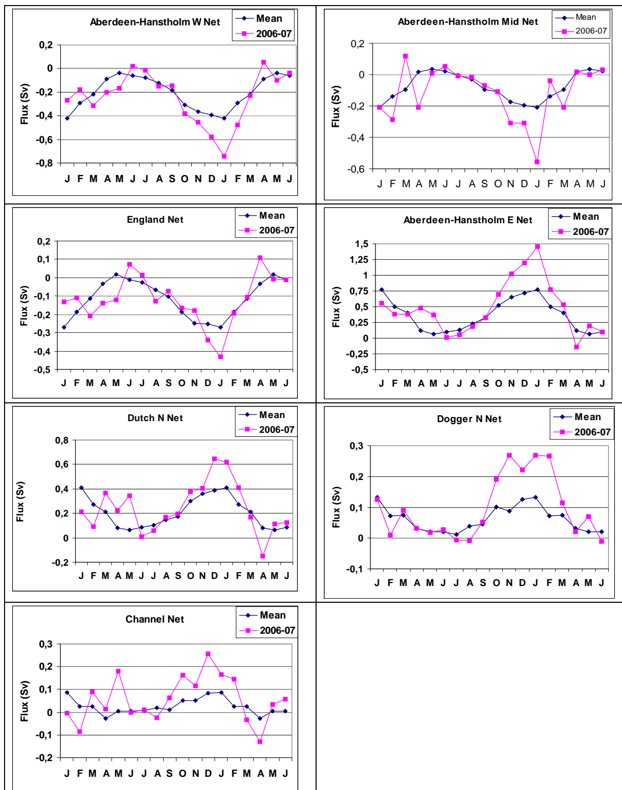
Figure 6. Modelled fluxes of water across sections in the central and southern North Sea (see Figure 2 for their locations). The mean monthly fluxes from January 2006 to June 2007 are shown along with the long-term mean (1955–2004) monthly fluxes. Net flux is the difference between northwards and southwards fluxes for transects oriented in the E-W direction, and between eastwards and westwards fluxes for transects oriented in the N-S direction. Negative values are southwards and westwards fluxes, while positive values are northwards and eastwards fluxes for E-W and N-S oriented sections, respectively.
